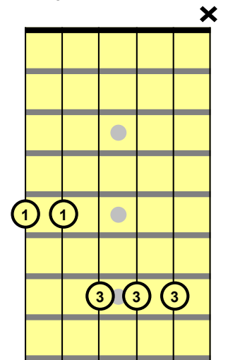
D power
